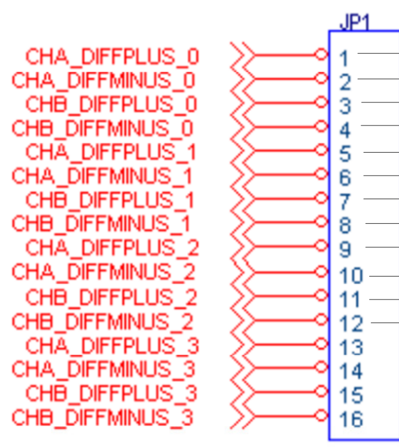
Terminal DIFF IN 0-3
