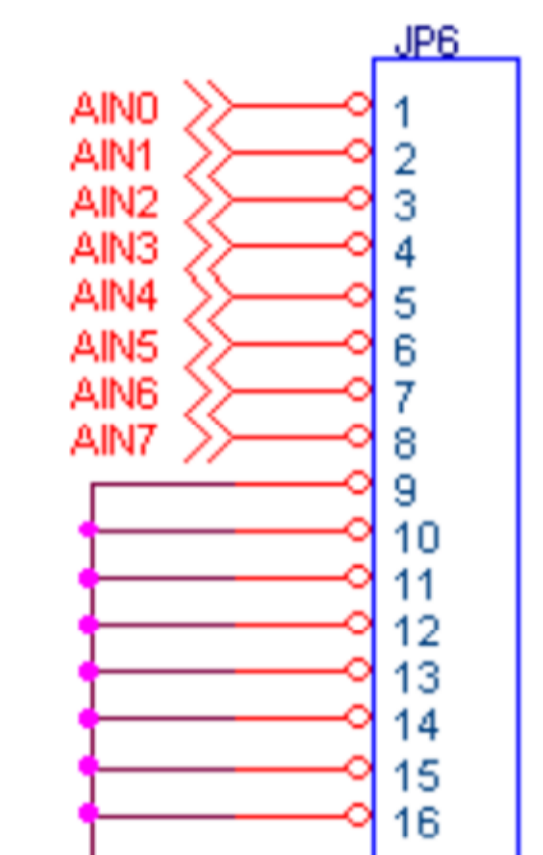
Terminal ADCs
